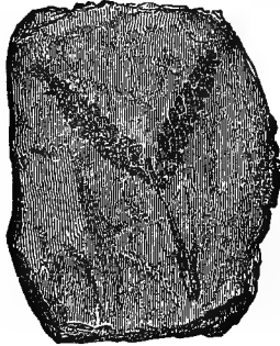
FERN? of Lower Old Red Sandstone. Orkney. (Nat. Size.)
